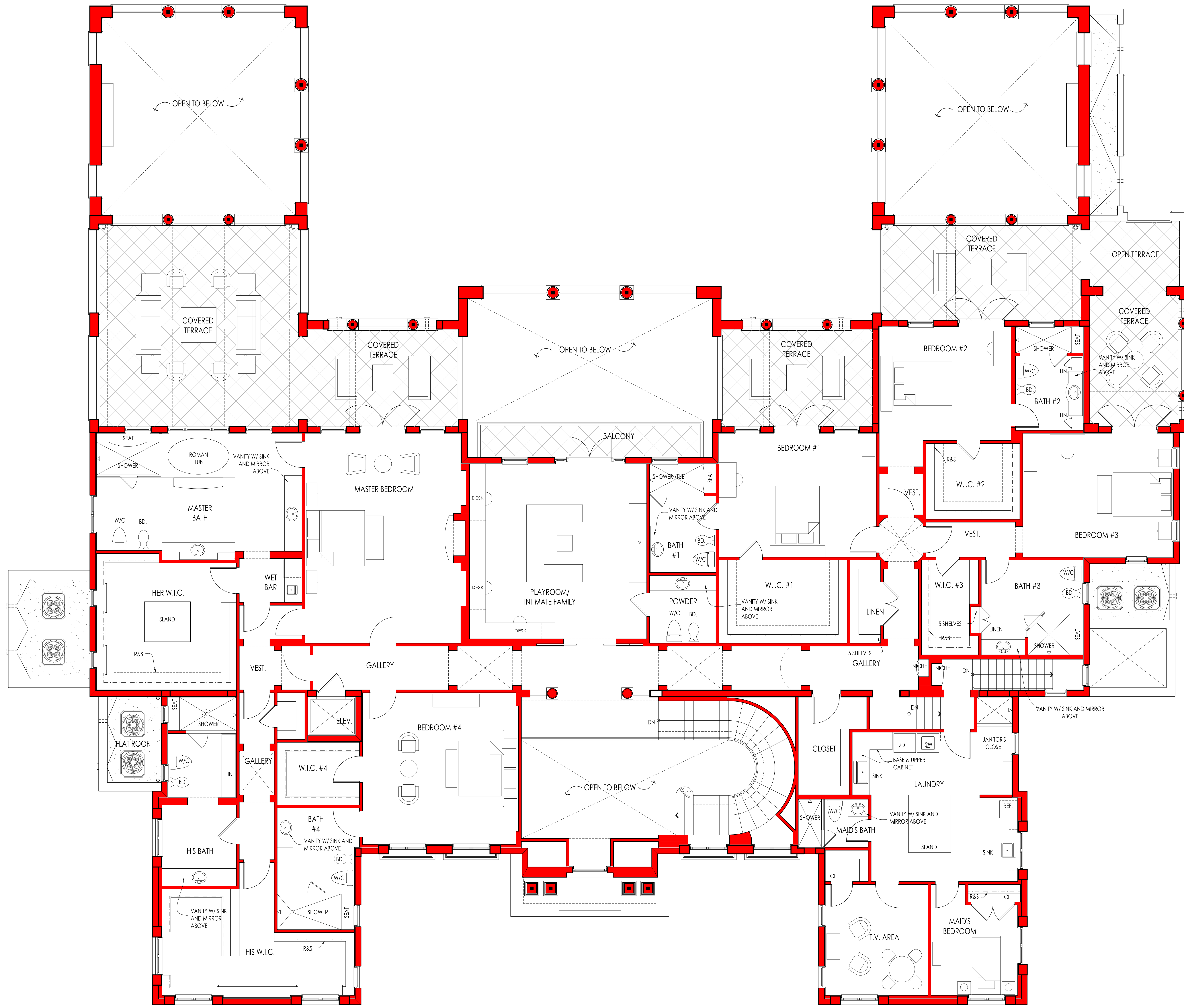
SECOND FLOOR PLAN SCALE 1/4" = 1'-0"
